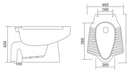
ANGLO INDIAN - S L 600 W 465 H 420mm
