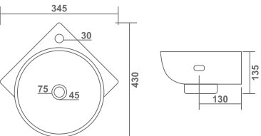
LEON CORNER L 430 W 345 H 135mm L 17" W 14" H 5"
