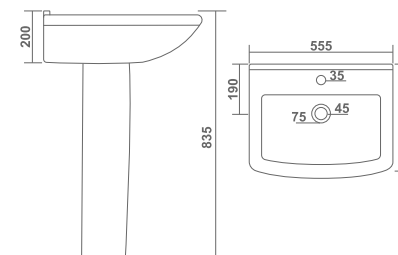
KAIZER SET L 480 W 555 H 835mm L 19" W 22" H 33"
