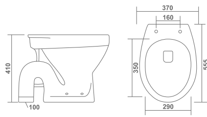
EWC - S L 555 W 370 H 410mm
