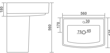
NEO HALF SET L 425 W 560 H 560mm L 17" W 22" H 22"
