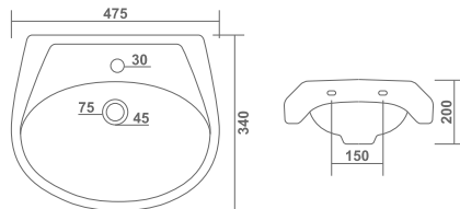
L 340 W 475 H 200mm DIAMOND L 14" W 19" H 8"
