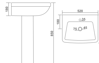
COSMO SET L 410 W 520 H 850mm L 16" W 21" H 34"
