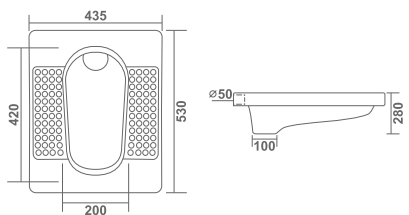
AQUA PAN L 530 W 435 H 280mm
