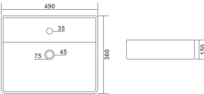
GLASSIA L 360 W 490 H 150mm L 14" W 20" H 6"
