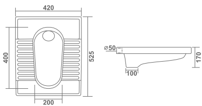
CITY PAN L 525 W 420 H 170mm
