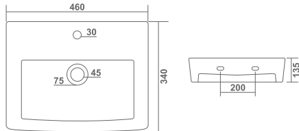
L 340 W 460 H 135mm SPARK L 14" W 18" H 5"
