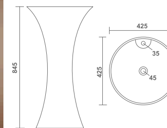
QUEENY L 425 W 425 H 845mm
