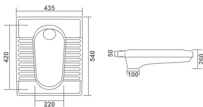
ORISSA PAN 20" L 540 W 435 H 260mm
