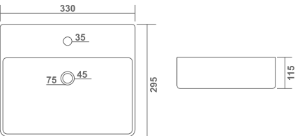
SLICE L 295 W 330 H 115mm L 12" W 13" H 5"
