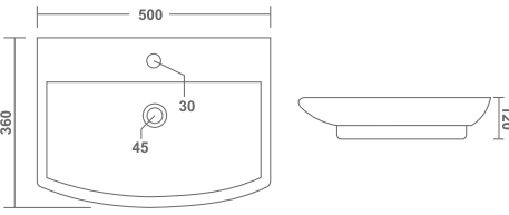
RIPON L 360 W 500 H 120mm L 14" W 20" H 5"
