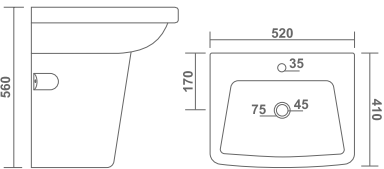
COSMO HALF SET L 410 W 520 H 560mm L 16" W 21" H 22"
