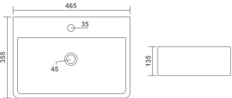
SOAR L 355 W 465 H 135mm L 14" W 19" H 5"
