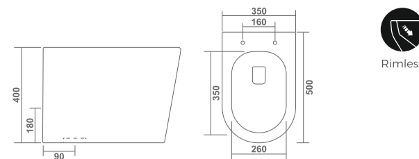
NEPTA L 500 W 350 H 400mm
