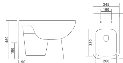
ALPINE L 545 W 345 H 450mm
