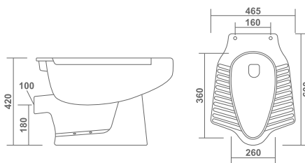
ANGLO INDIAN - P L 600 W 465 H 420mm
