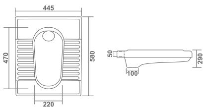
ORISSA PAN-23" L 580 W 445 H 290mm
