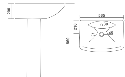
L 460 W 565 H 860mm SQUARE SET L 18" W 23" H 34"
