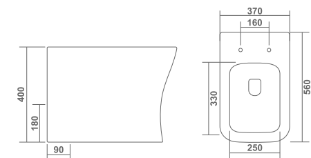
SAHARA L 560 W 370 H 400mm
